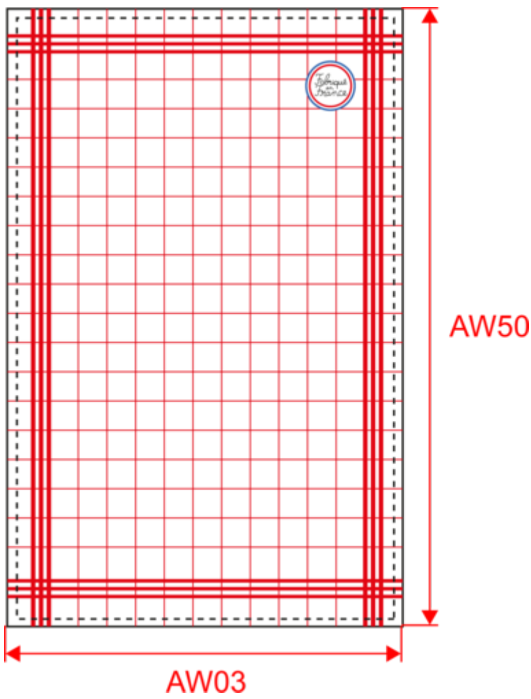
Dimensions (cm)
